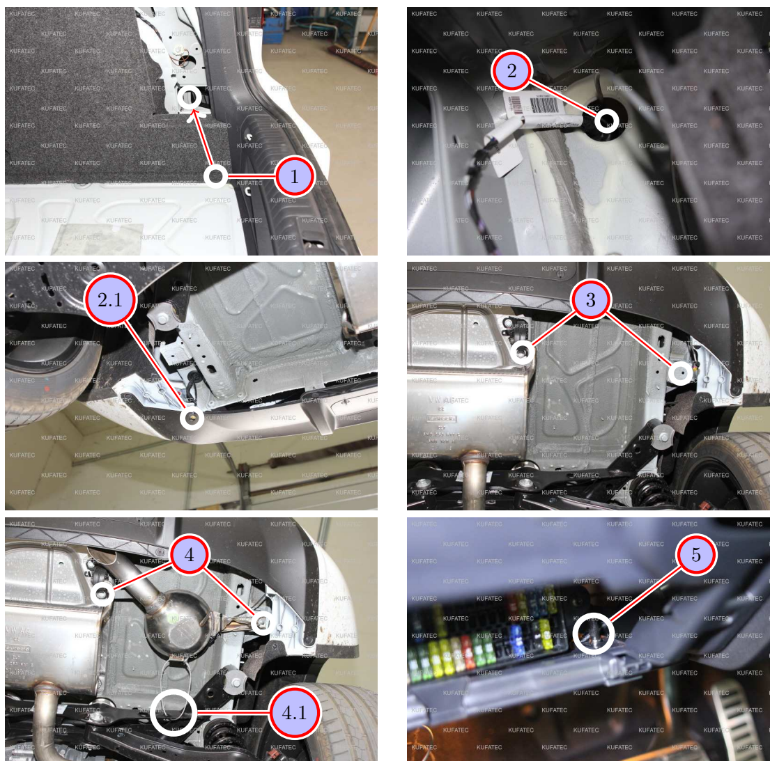
Figure 8: Installation soundbooster and pushbutton
