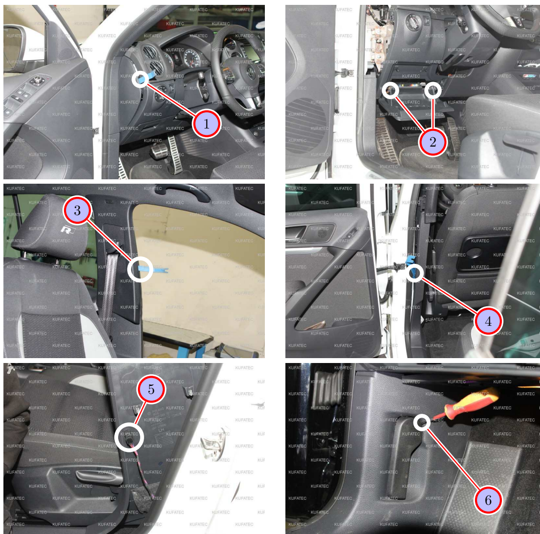
Figure 4: Removing trim panels front
