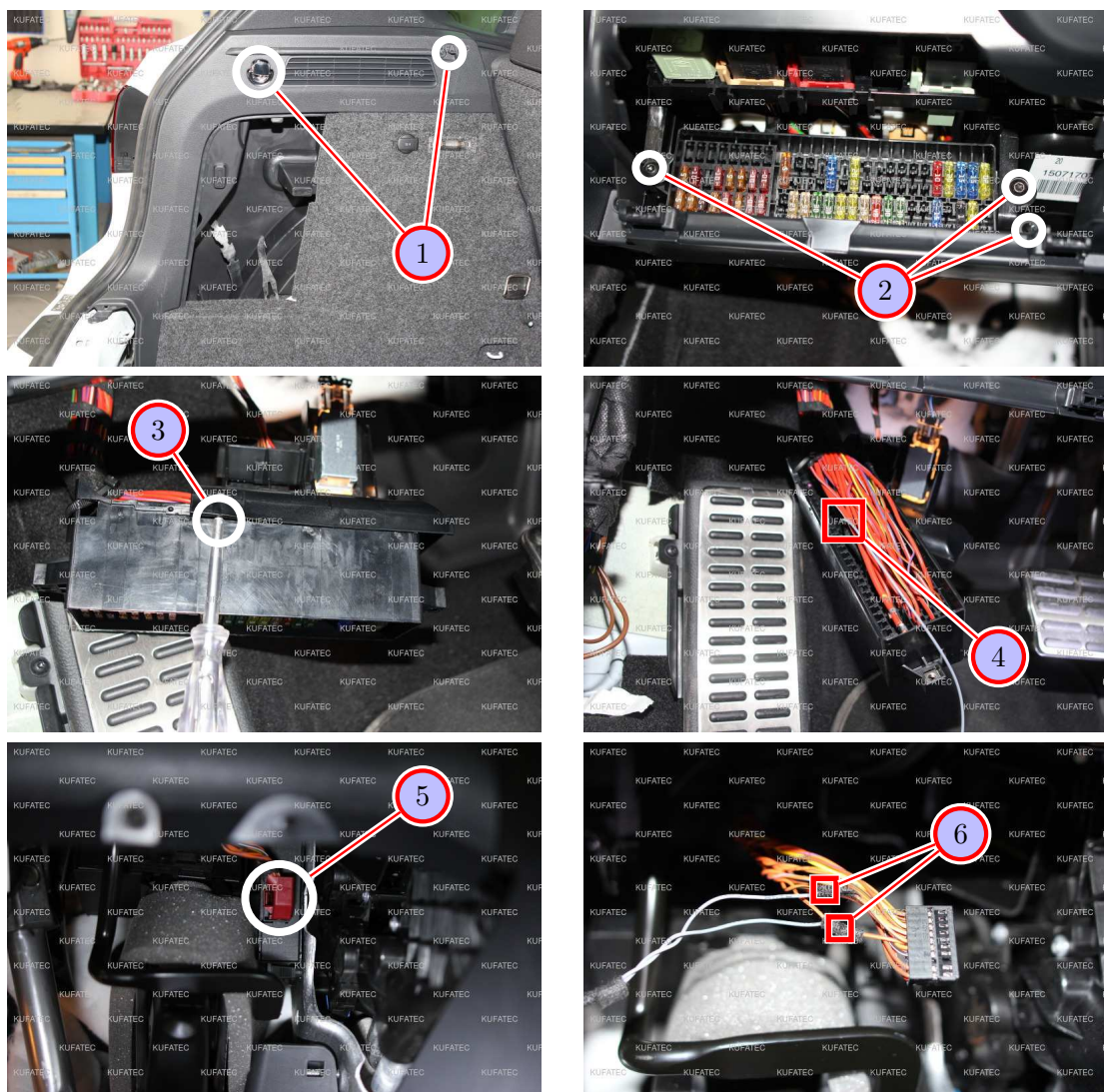
Figure 6: Connection power supply and CAN-Bus
