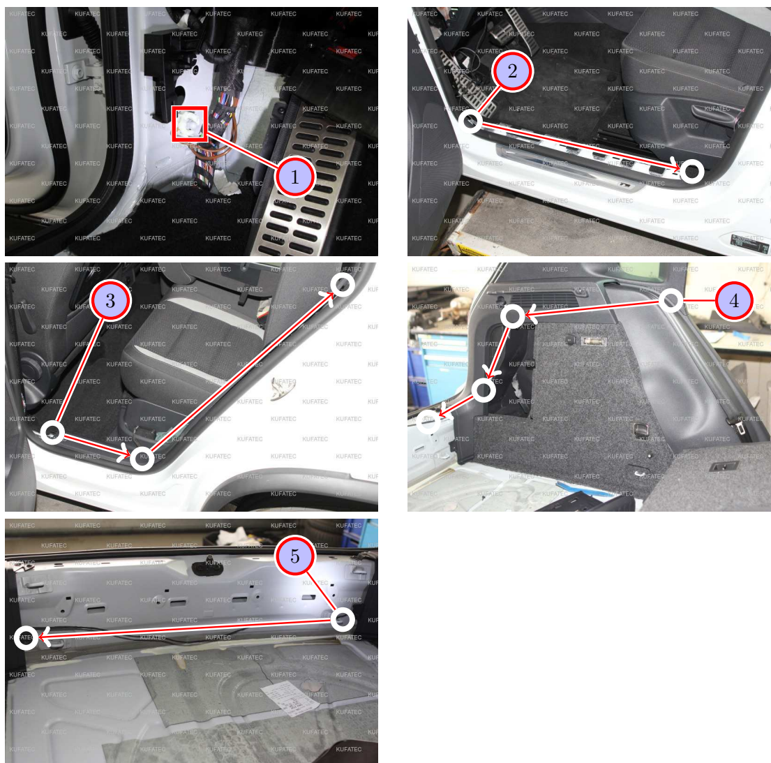
Figure 7: Connection ground and cable routing in the trunk
