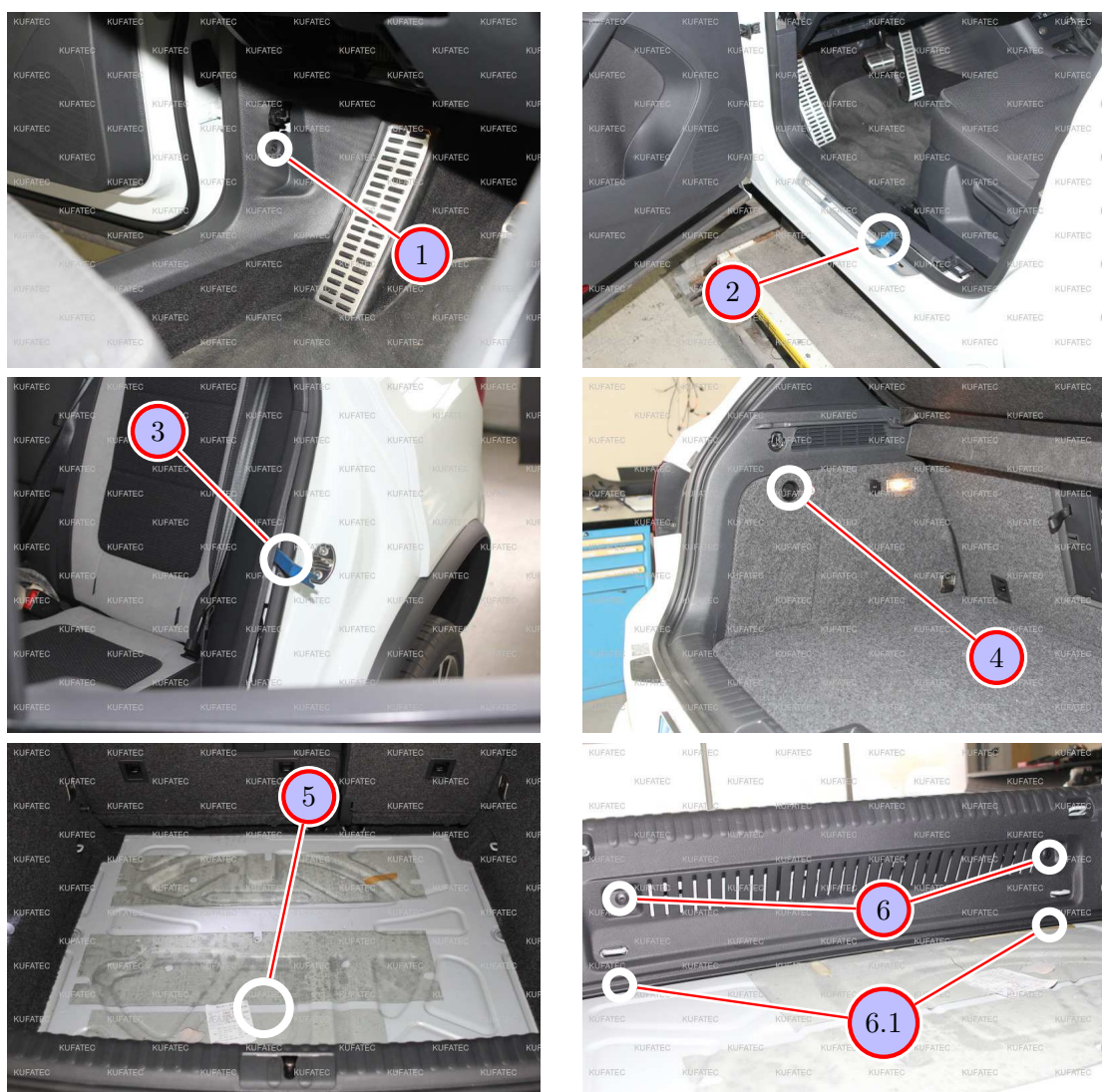
Figure 5: Removing front sill trim and trunk sill covering
